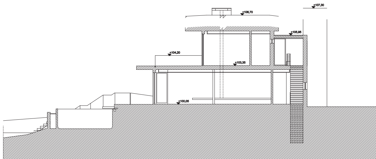
SECTIONS BB' | CORTE BB'
