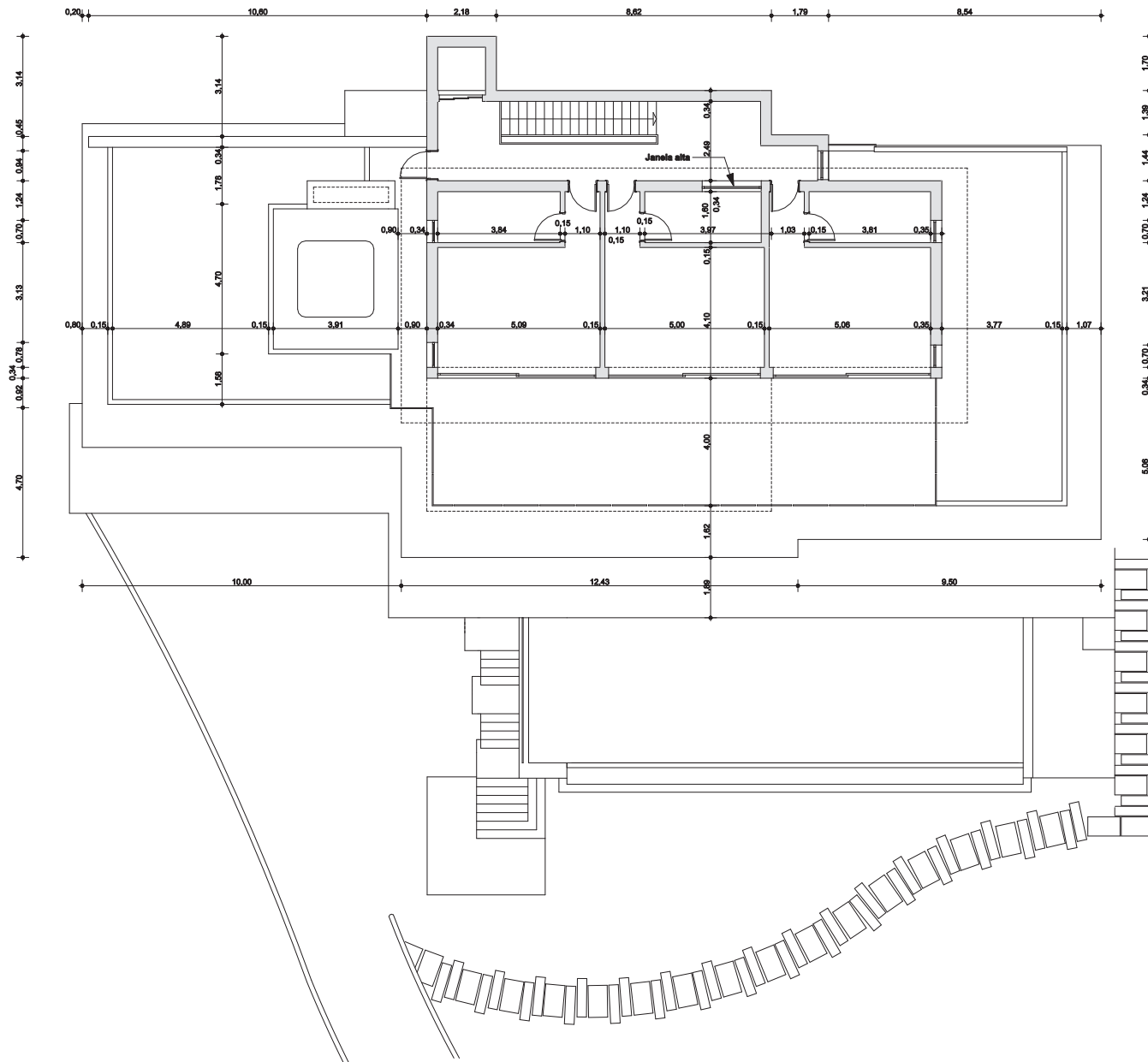
1st FLOOR | 1° ANDAR
