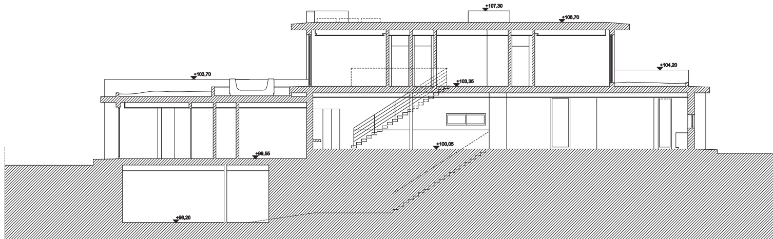
SECTIONS AA' | CORTE AA'
